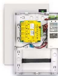
Net2 I/O board - 12V 2A PSU, Plastic cabinet
